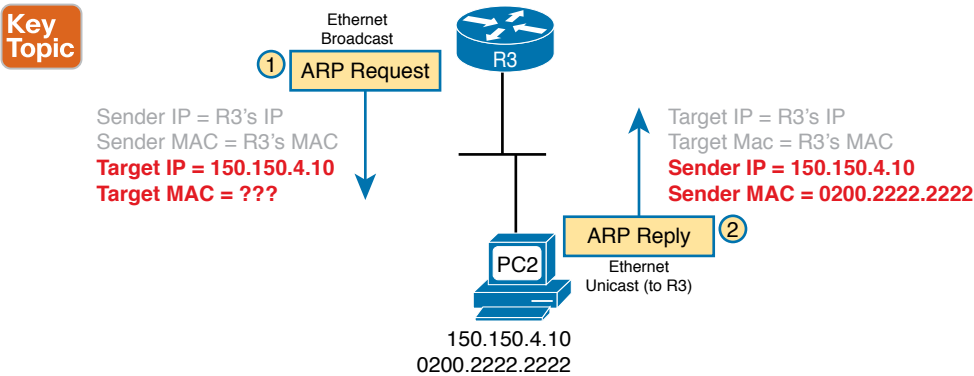
Figure 3-15 Sample ARP Process
