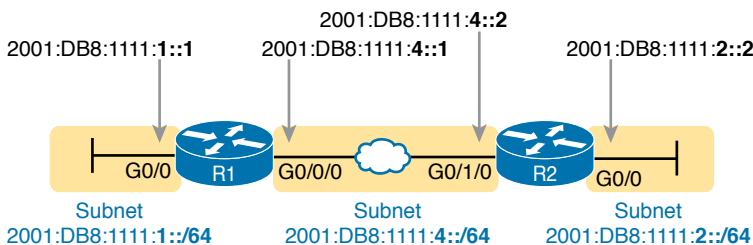
Figure 24-3 Sample 128-bit IPv6 Addresses to Be Configured on Cisco Router Interfaces
