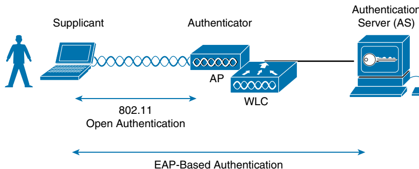
Figure 28-6 802.1x Client Authentication Roles
