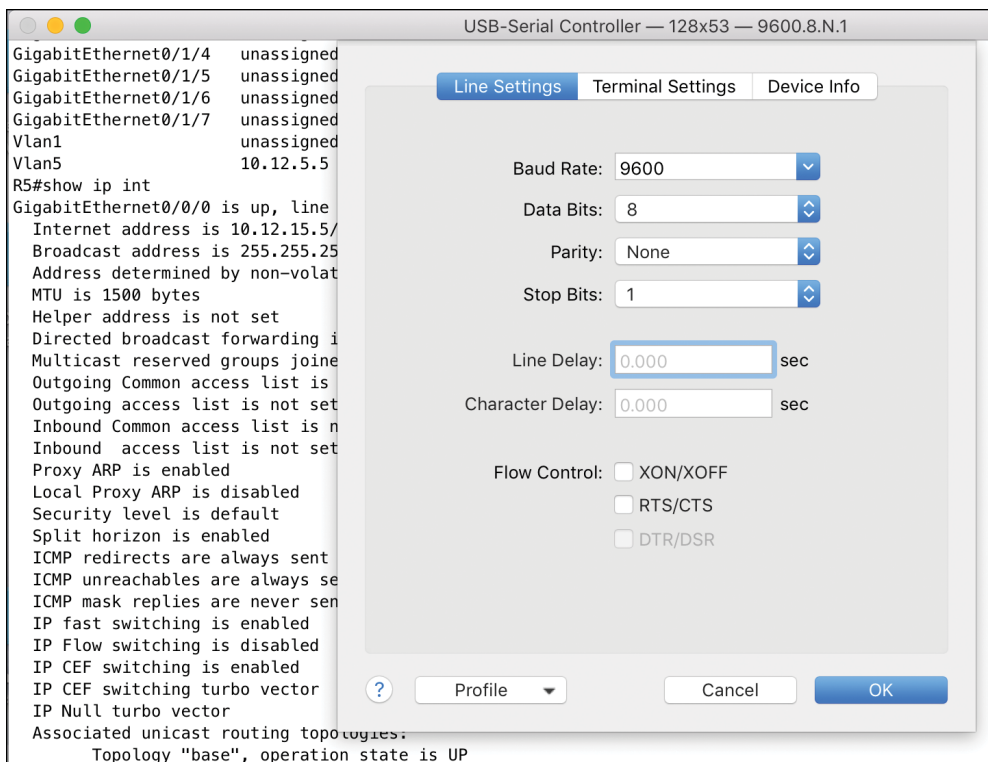
Figure 4-5 Terminal Settings for Console Access
