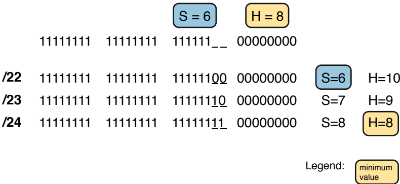
Figure L-6 Three Masks That Meet the Requirements
