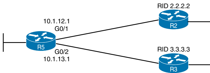
Figure 21-5 Example Network to Demonstrate OSPF Process Shutdown
