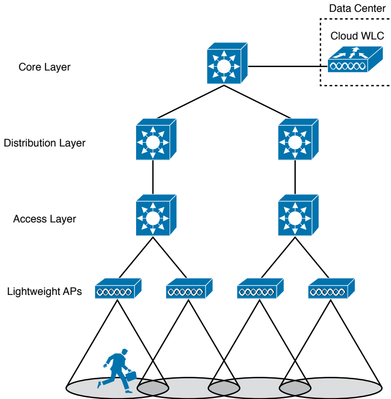
Figure 27-9 WLC Location in a Cloud-based Deployment
