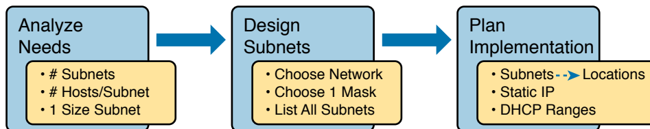
Figure L-1 Subnet Design and Implementation Process from Chapter 11
