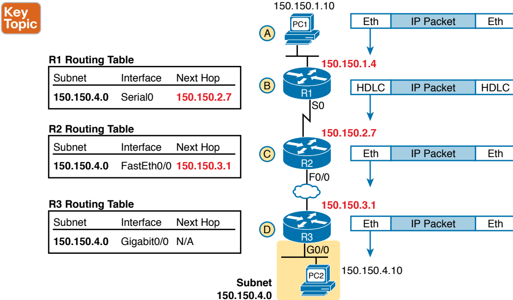
Figure 3-11 Network Layer and Data-Link Layer Encapsulation
