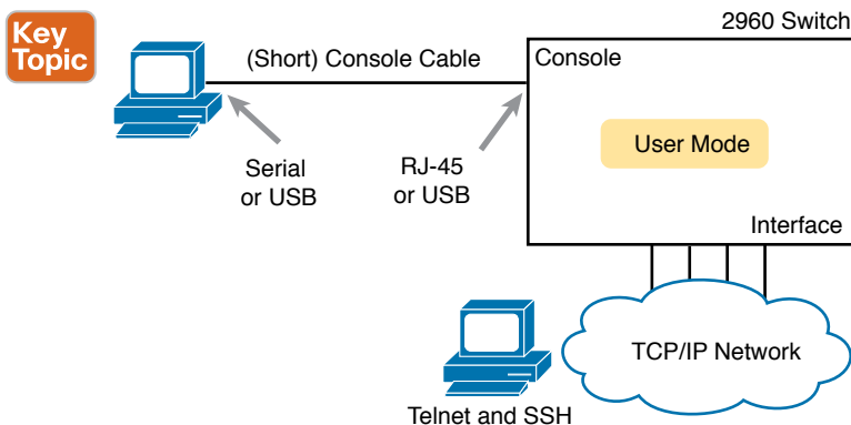
Figure 4-2 CLI Access Options
