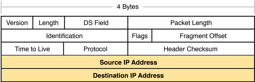
Figure 3-12 IPv4 Header, Organized as 4 Bytes Wide for a Total of 20 Bytes
